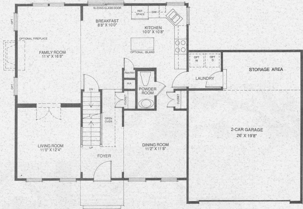
FIRST FLOOR
