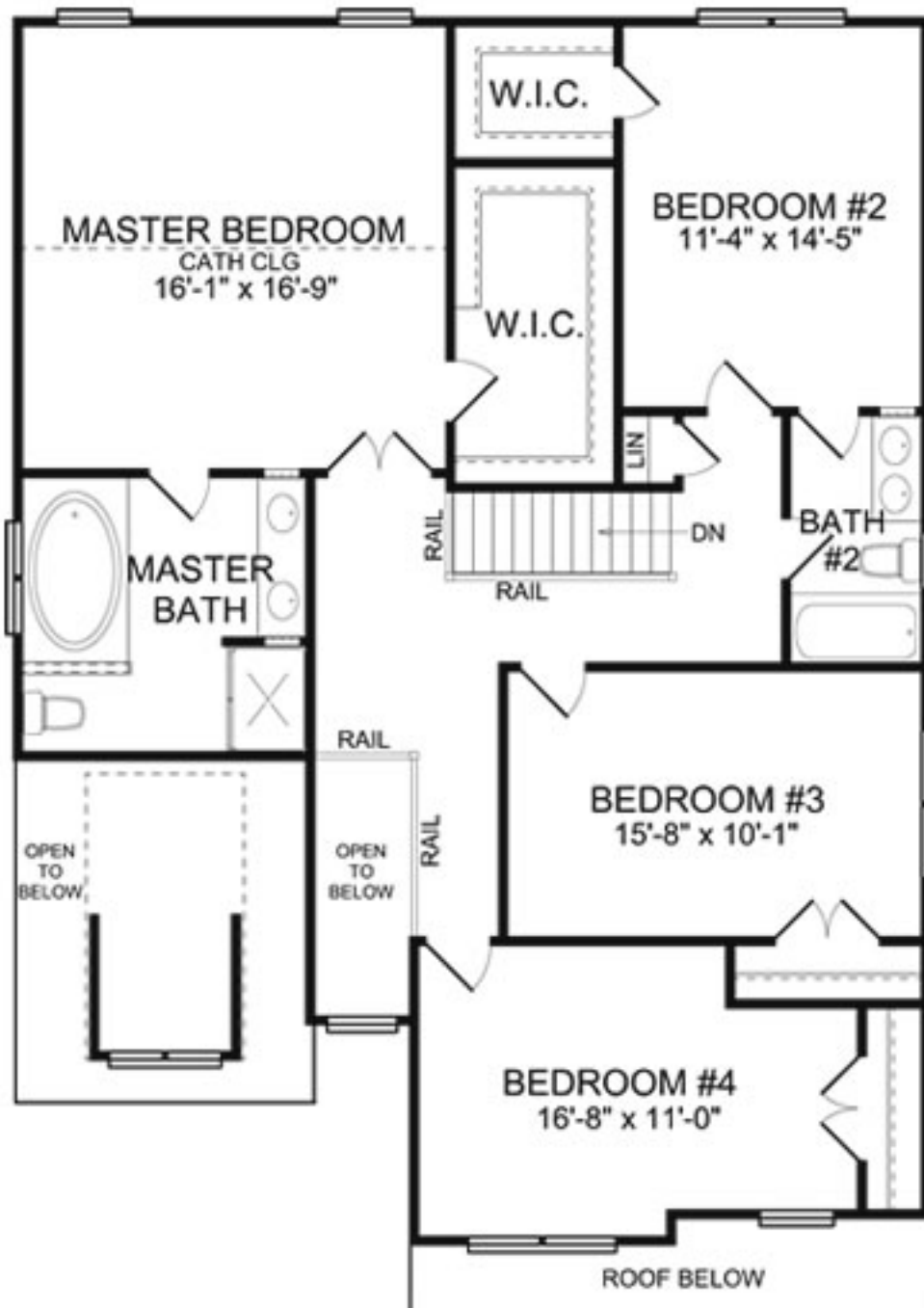
SECOND FLOOR PLAN THE BANNEKER
